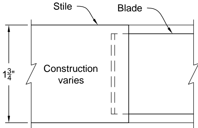
LOUVER DETAIL @ STILE TYPICAL 1 3/4" LOUVER DOOR
