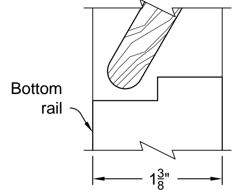
LOUVER DETAIL @ TOP & BOTTOM RAIL 1-3/8" LOUVER DOOR
