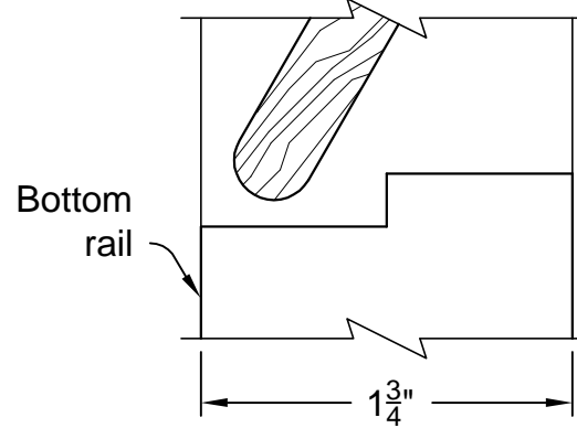
LOUVER DETAIL @ TOP & BOTTOM RAIL 1-3/4" LOUVER DOOR
