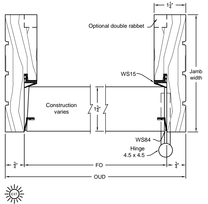
TYP. JAMB DETAIL SECTION 1-3/4" EXT. OUTSWING DOOR
