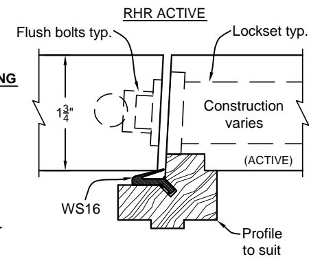
TYP. ASTRAGAL DETAIL EXTERIOR DOUBLE DOORS
