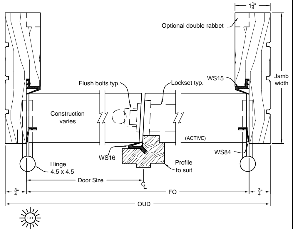
TYP. JAMB DETAIL SECTION EXTERIOR DBL. DOOR (RHR, Active Shown)
