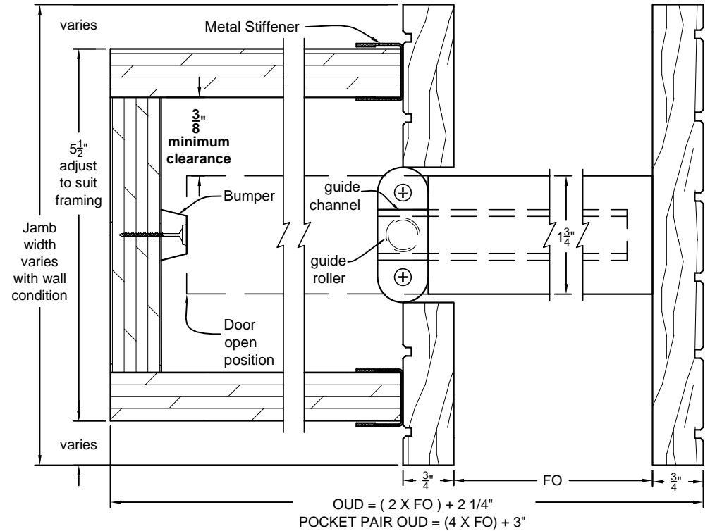
TYP. JAMB DETAIL SECTION POCKET DOOR - 5-1/2" CAGE wo/STOPS
