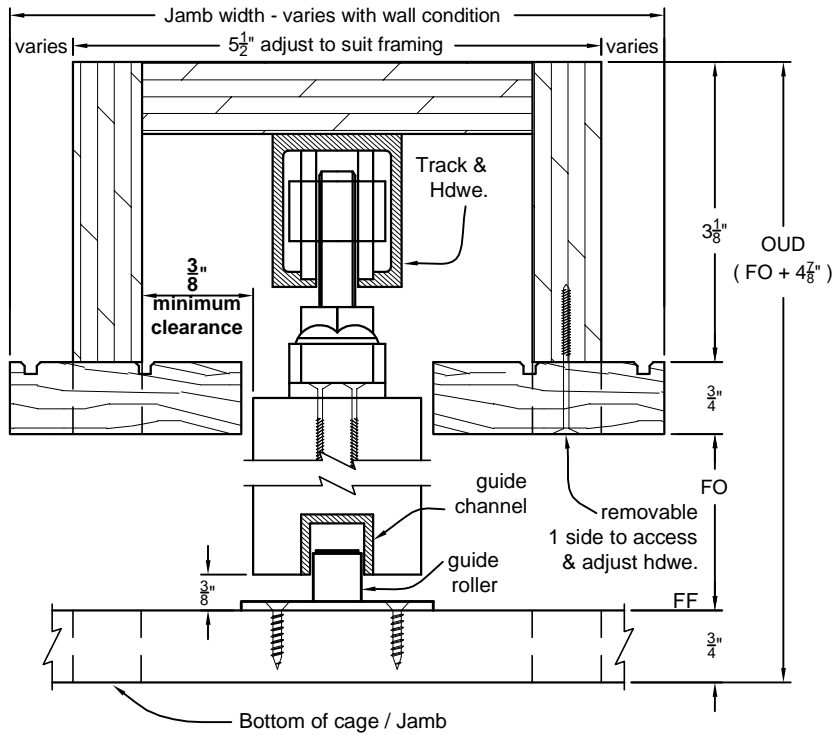
TYP. HEAD & SILL DETAIL SECTION POCKET DOOR - 5-1/2" CAGE wo/STOPS
