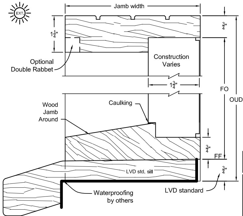
TYP. HEAD & SILL SECTION 1-3/4" (2-1/4" Thick Sim.) EXT. FIXED SIDELITE @ INSWING DOOR
