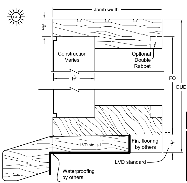
TYP. HEAD & SILL SECTION 1-3/4" (2-1/4" Thick Sim.) EXT. FIXED SIDELITE @ OUTSWING DOOR
