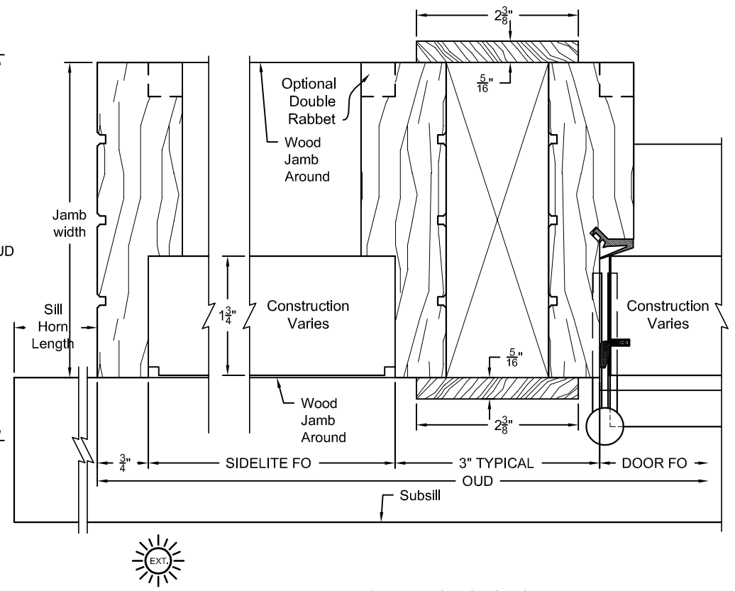
TYP. JAMB & MULLION SECTION 1-3/4" (2 -1/4" Thick Sim.) EXT. FIXED SIDELITE @ OUTSWING LH DOOR
