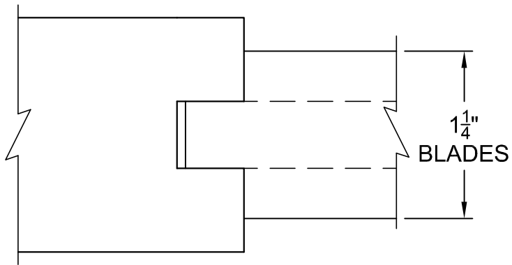
FALSE LOUVER DETAIL @ STILE
