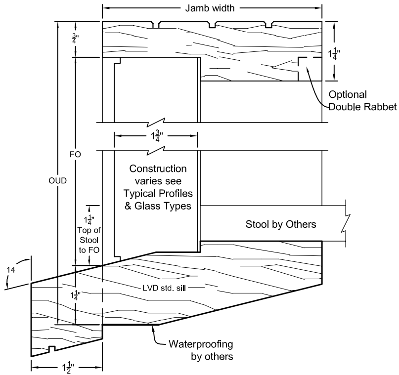
TYP. HEAD & SILL SECTION 1-3/4" FIXED WINDOW OR TRANSOM
