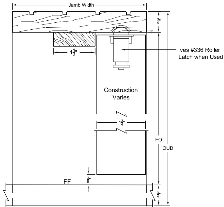
TYP. HEAD & SILL SECTION INTERIOR DOOR
