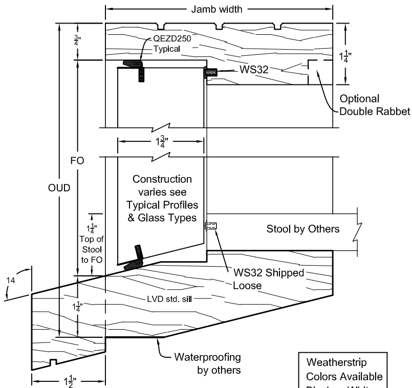
TYP. HEAD & SILL SECTION 1-3/4" OUTSWING AWNING WINDOW
