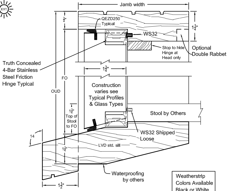
TYP. HEAD & SILL SECTION 1-3/4" OUTSWING CASEMENT WINDOW
