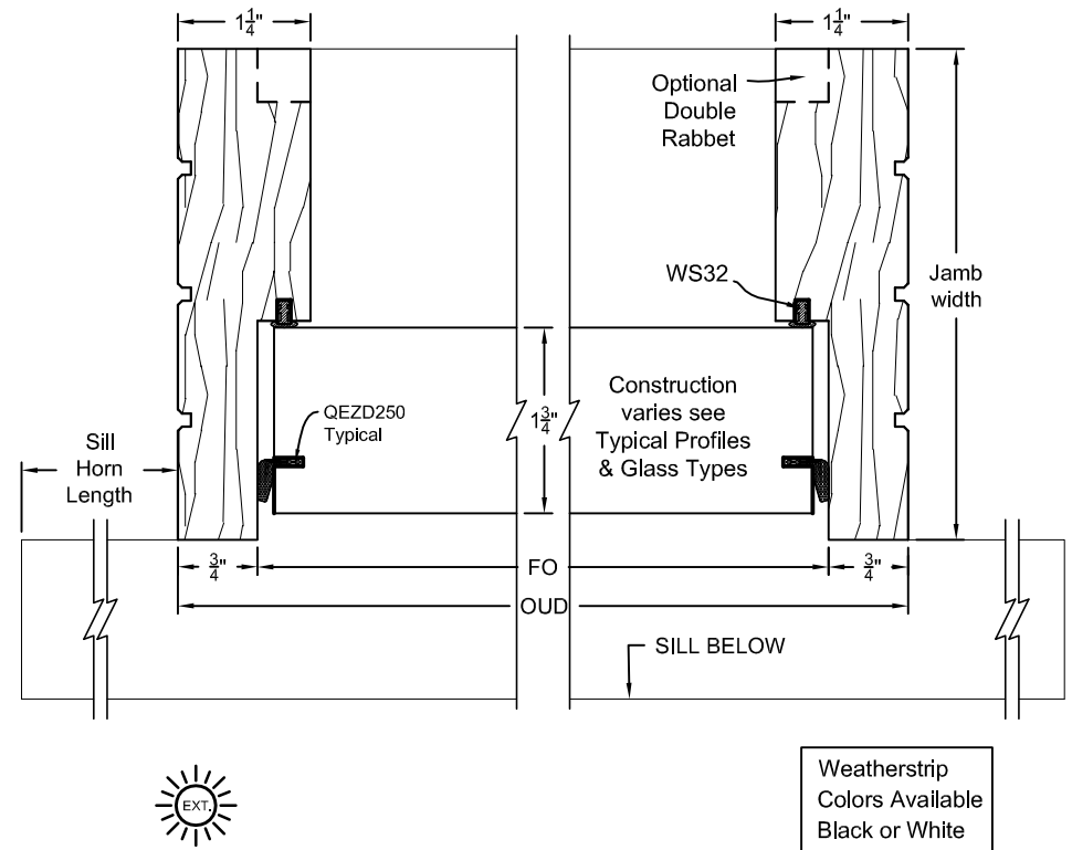
TYP. JAMB SECTION 1-3/4" OUTSWING CASEMENT WINDOW
