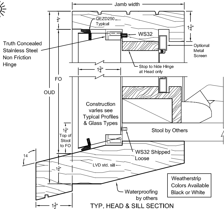
TYP. HEAD & SILL SECTION 1-3/4" CASEMENT WINDOW w/ CRANK & OPTIONAL SCREEN
