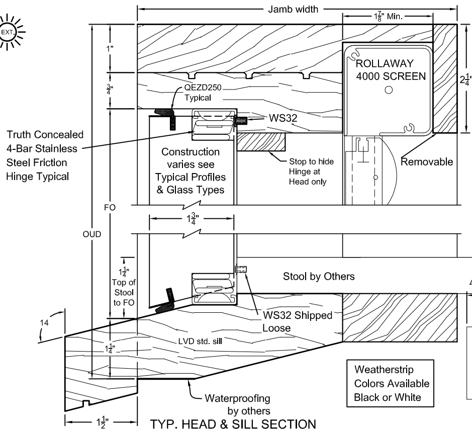
1-3/4" OUTSWING CASEMENT WINDOW WITH HIDDEN ROLLAWAY SCREEN
