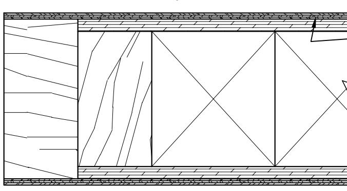
LVD ENGINEERED CORE FLUSH DOOR
