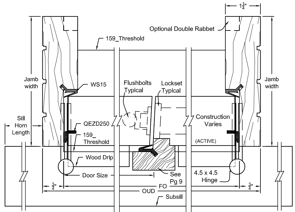
TYP. OUTSWING ASTRAGAL SECTION EXTERIOR PAIR DOOR (RHR, Active Shown) SEE PG 9 FOR ASTRAGAL PROFILE OPTIONS
