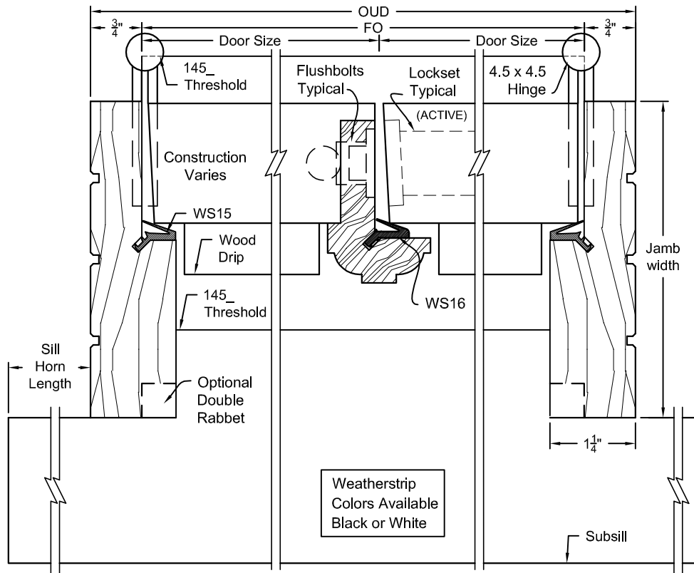
TYP. INSWING ASTRAGAL SECTION EXTERIOR PAIR DOOR (RH, Active Shown) SEE PG 9 FOR ASTRAGAL PROFILE OPTIONS
