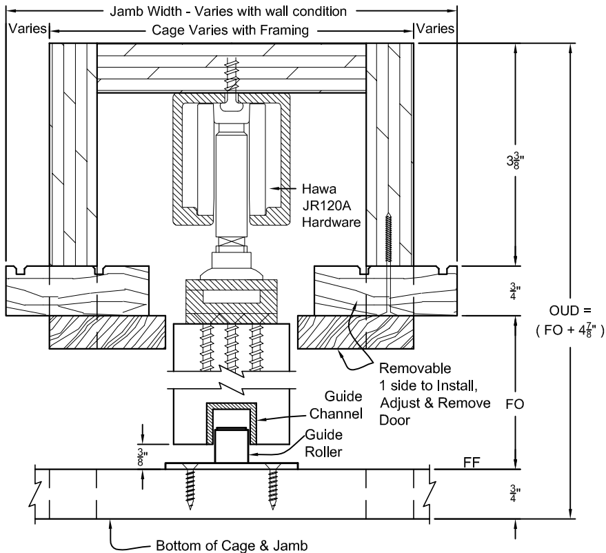
TYP. HEAD & SILL SECTION POCKET FRAME - HAWA 120A HARDWARE - WITH STOPS
