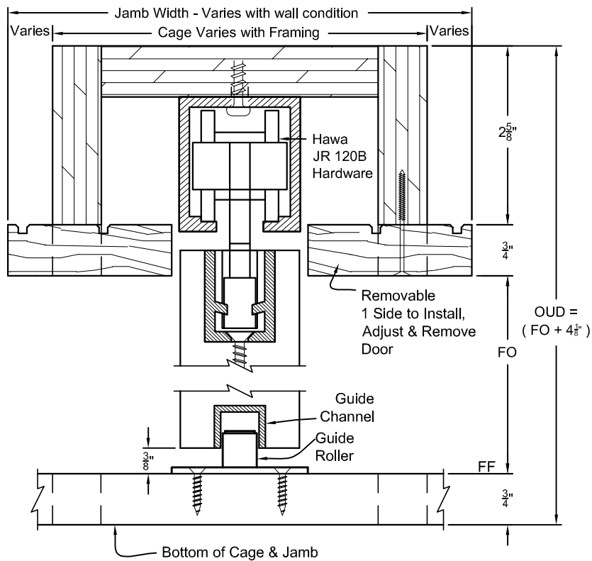
TYP. HEAD & SILL SECTION POCKET FRAME - HAWA 120B HARDWARE - STOPLESS
