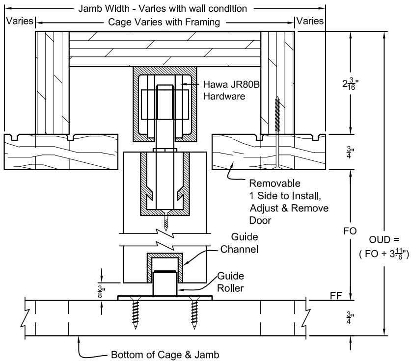
TYP. HEAD & SILL SECTION POCKET FRAME - HAWA 80B HARDWARE - STOPLESS
