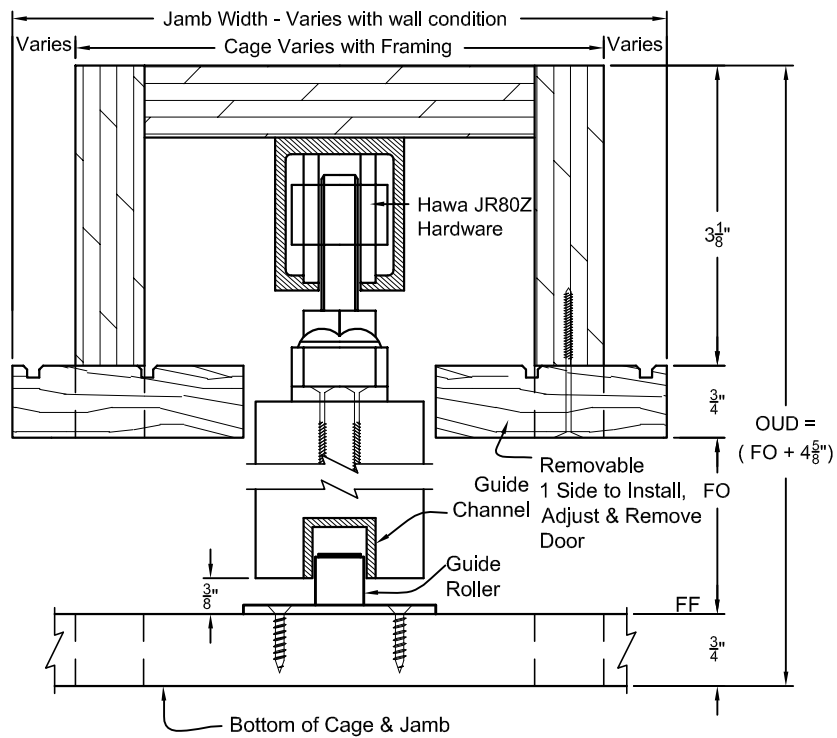
TYP. HEAD & SILL SECTION POCKET FRAME - HAWA 80Z HARDWARE - STOPLESS
