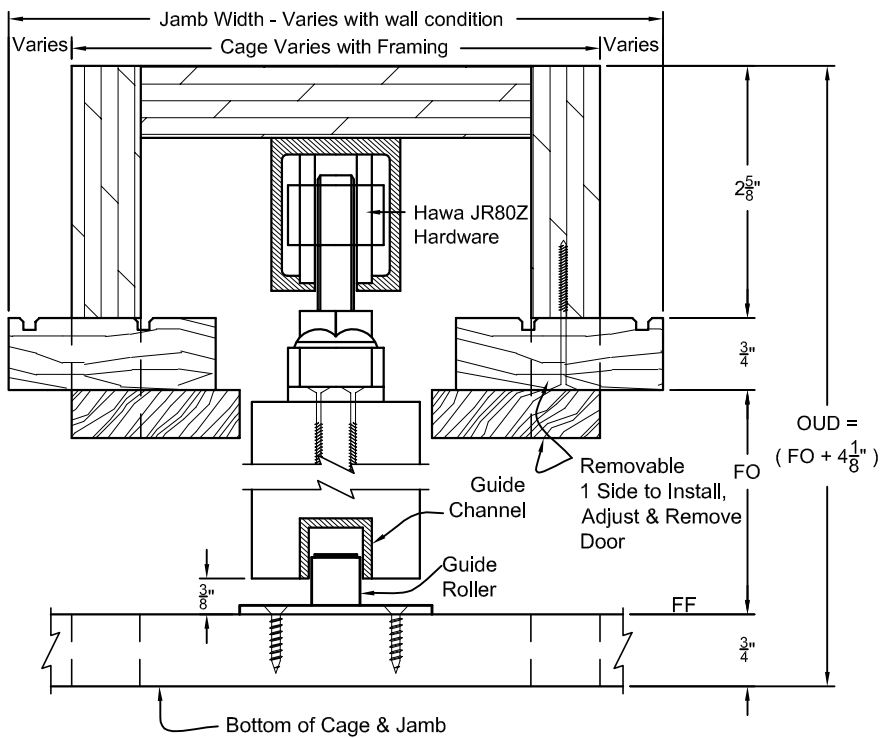
TYP. HEAD & SILL SECTION POCKET FRAME - HAWA 80Z HARDWARE - WITH STOPS
