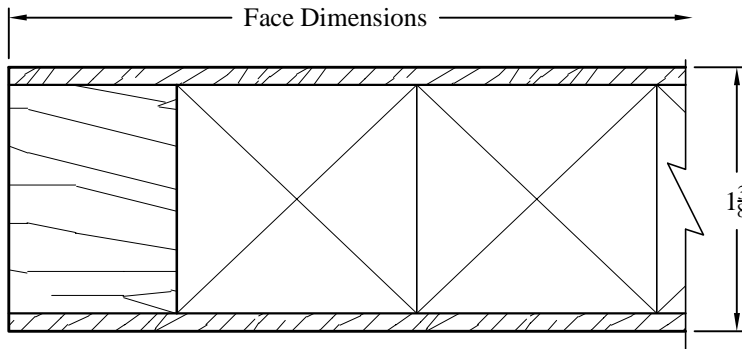
ENGINEERED/ VENEER STILE & RAIL Pine Core @ interior
