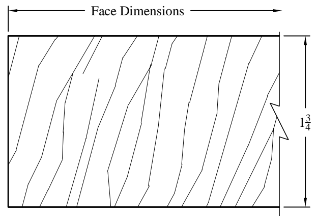
SOLID STOCK STILE & RAIL
