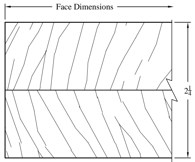
2 PLY LAMINATED STILE & RAIL
